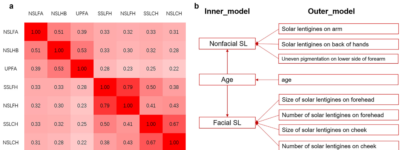
Supplementary Figure S2. Pearson correlation among seven SL traits and composite phenotype extraction of facial SLs. (a) Pearson correlation among seven SL phenotypes. (b) Composite phenotype extraction by partial least square path model. NSLCH, number of solar lentigines on the cheek; NSLFA, solar lentigines on the forearm; NSLFH, number of solar lentigines on the forehead; NSLHB, solar lentigines on the back of the hand; SL, solar lentigines; SSLCH, size of solar lentigines on the cheek; SSLFH, size of solar lentigines on the forehead; UPFA, uneven pigmentation on the lower side of the forearm.
